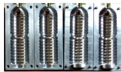
Three Sets Mould (300ml-500ml-1000ml)
